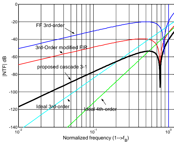
Fig. 3. The magnitude responses of the 3rd , 4th-order NTFs with various type.
