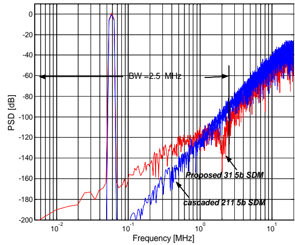
Fig. 4. The ideal output spectra of \Sigma\Delta modulators.
