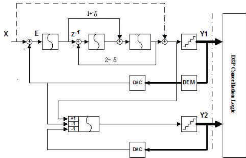
Fig. 2. Proposed 4th-order cascade 3(4b)-1(5b) \Sigma\Delta Modulator.
